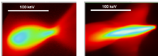
Figure 8: Dark current (left) and electron beam (right) images in the dispersive beamline behind the 180^\circ dipole.
