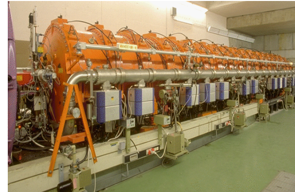
Single Gap Resonators
