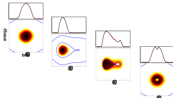
Figure 5: Longitudinal bunch merging using the h = 8 and h = 16 RF systems at the CERN PS.
