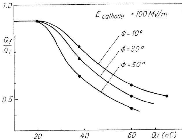
Fig. 2 : The survival rate Q_f/Q_i as function of the initial charge Q_i of the bunch ( t = 30 \text{ ps} , j = 84/\text{mm}^2 ) for different rf-phases.
