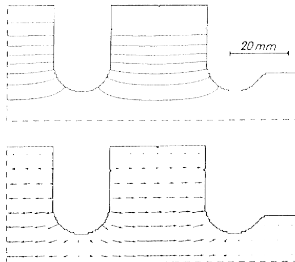
Fig. 1: Field patterns ( H\phi \cdot r = \text{const.} , E ) of the 3 GHz 1 1/2 cell rf-gun oscillating in \pi -mode; the cathode is located on the left side.
