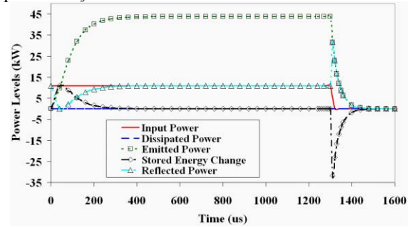
Figure 6: System power response versus the time.
