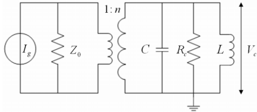
Figure 5: Equivalent circuit model of the coupling system.
