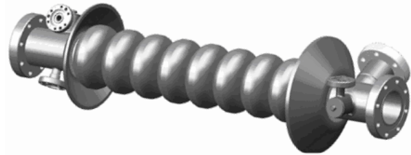
Figure 1: A naked third harmonic superconducting cavity.
